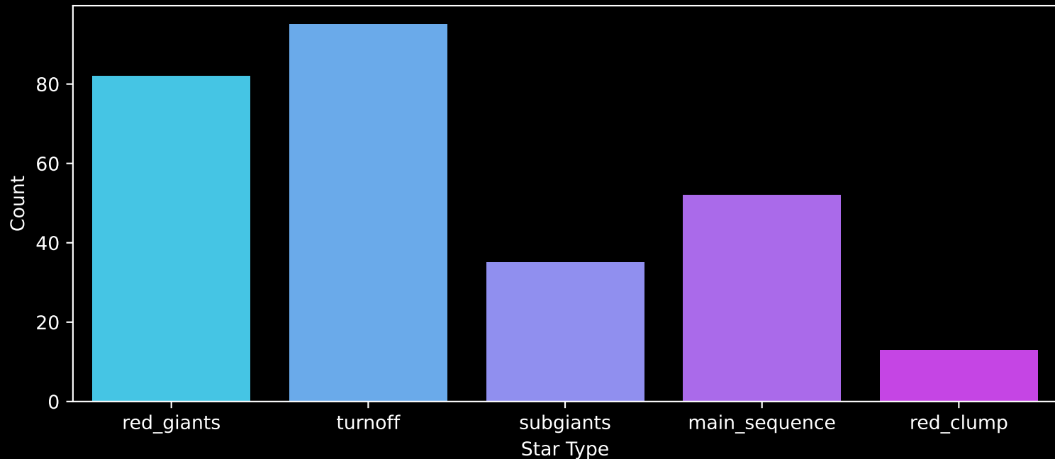
GALAH DR4 Field: [8960] Count plot of Star Type
