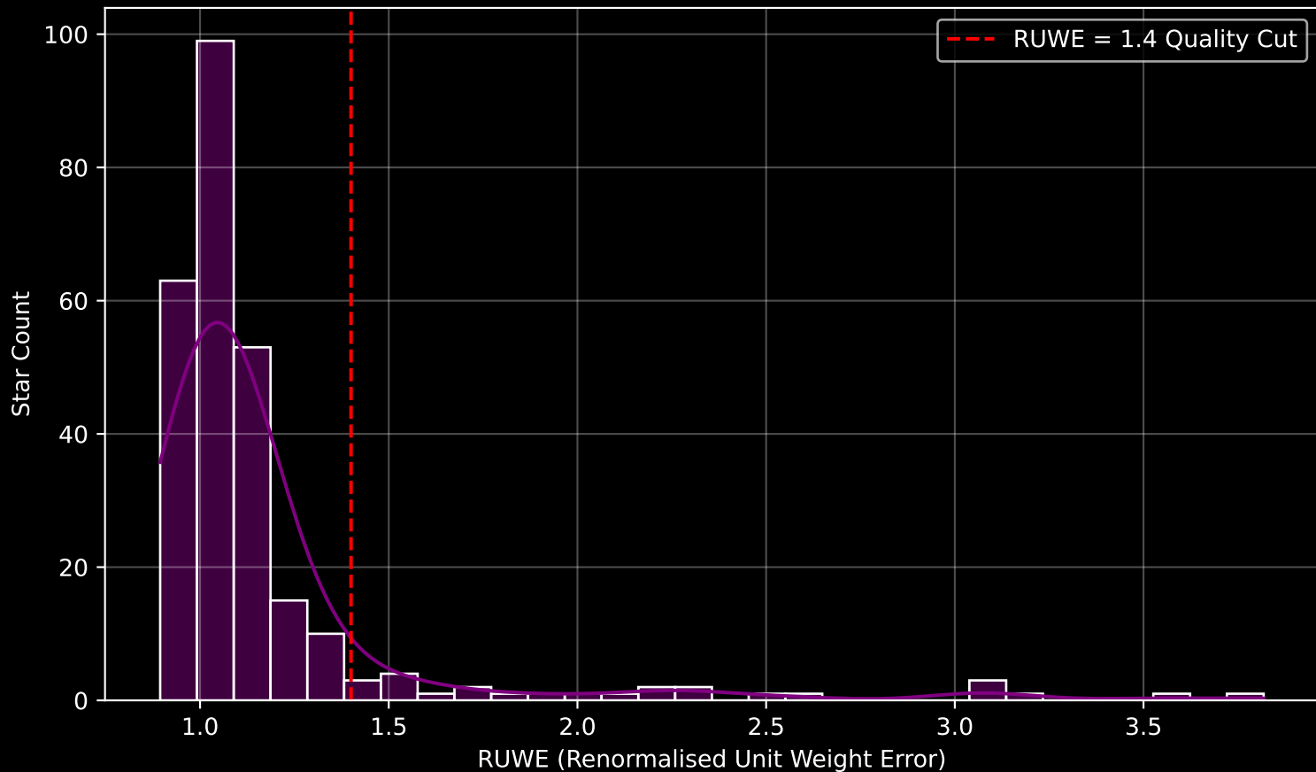
GALAH DR4 Field [8960] RUWE Distribution (n= 266)
