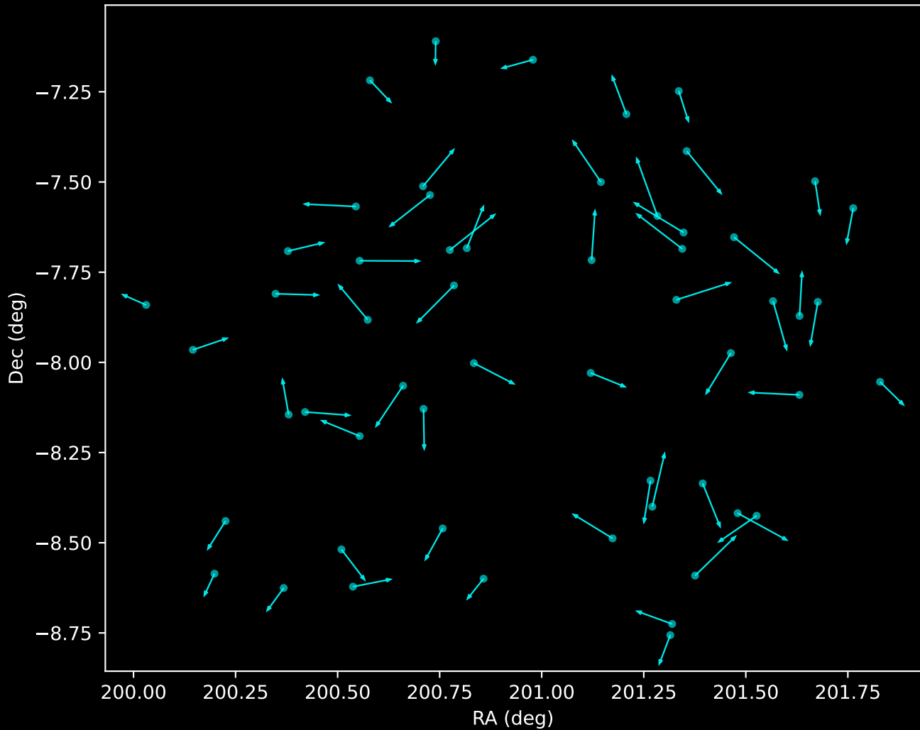
GALAH DR4 Noise Stream Proper Motion Vectors (n=56)
