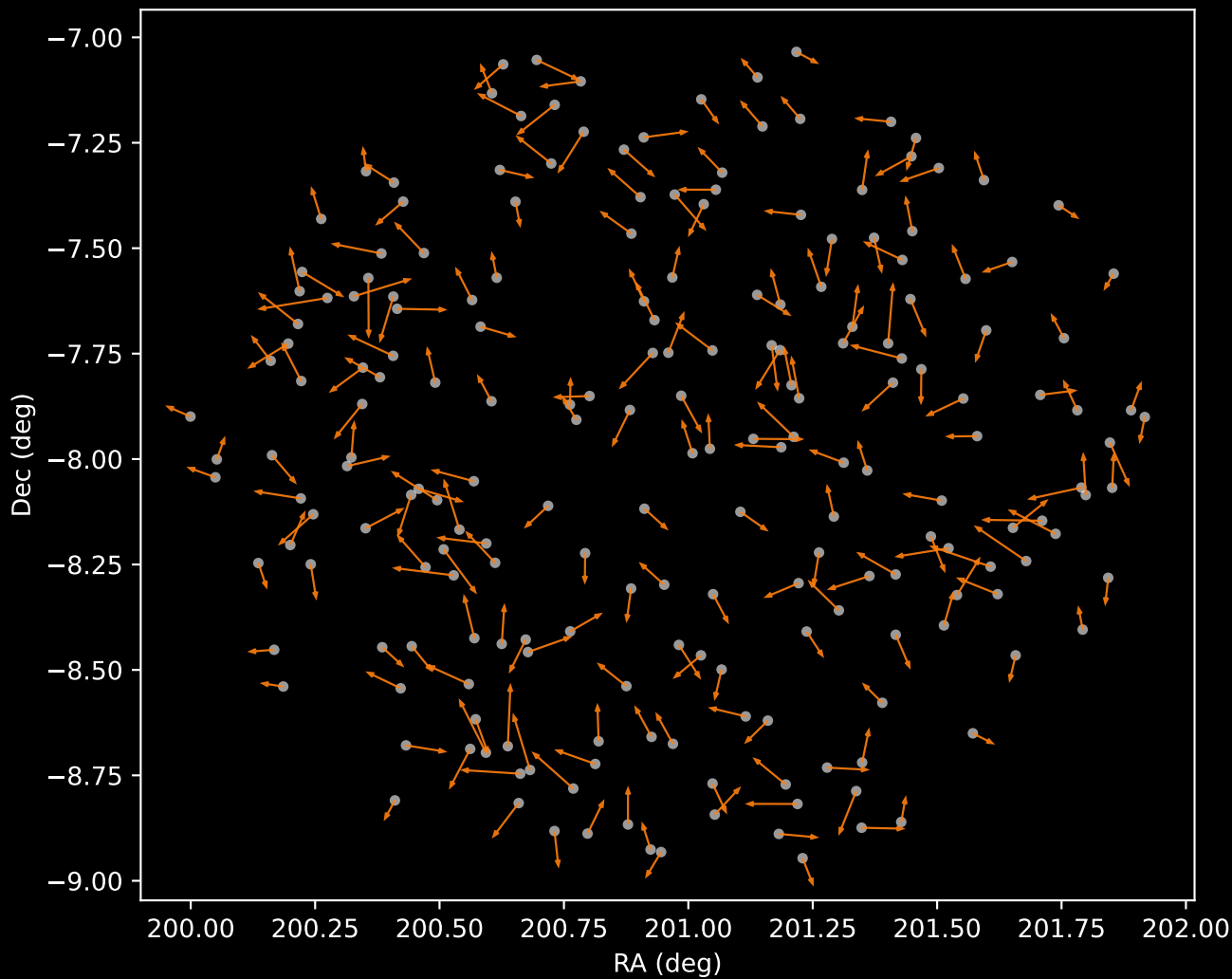
GALAH DR4 Cluster 2 Proper Motion Vectors (n=208)
